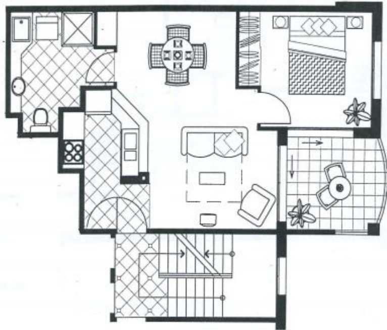
MIDDLE AND GROUND LEVEL – TYPICAL 1 BEDROOM APARTMENT
